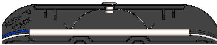
DETAIL A (EXTENDED) SCALE 1 : 1 SPRING CLAMP SHOWN FLEXED WITH A COUPLER HOUSING IN PLACE
