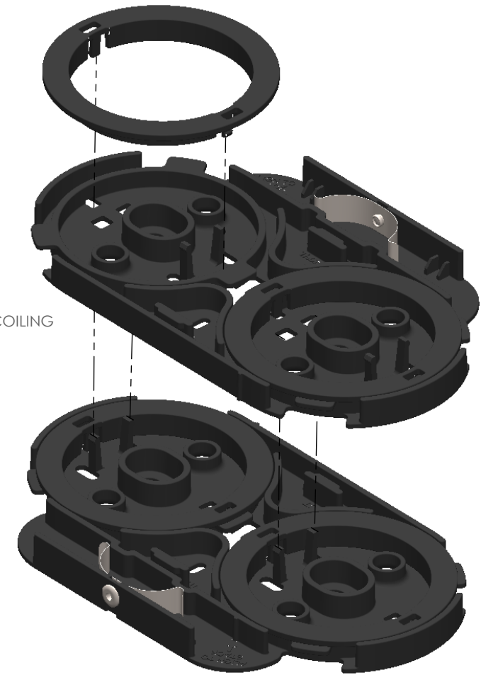
EXPLODED ISOMETRIC VIEW SHOWING ONE LID AND TWO TRAYS IN STACKING ALIGNMENT
